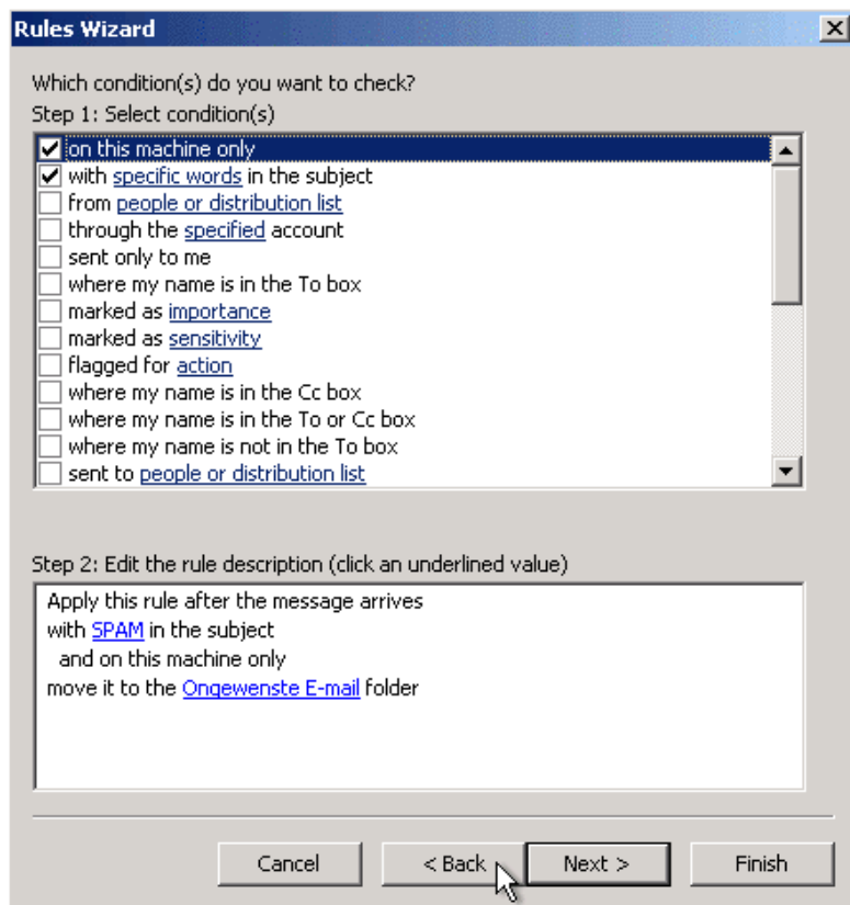
Figure 5.13. Rules wizard
