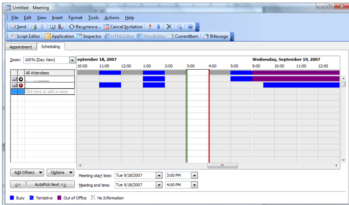
Figure 5.10. Free/Busy information
