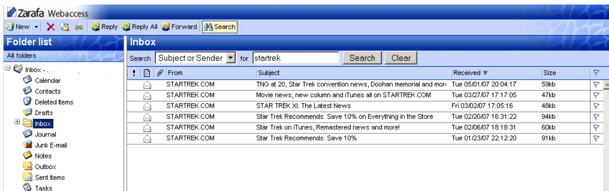
Figure 2.22. Search Result
