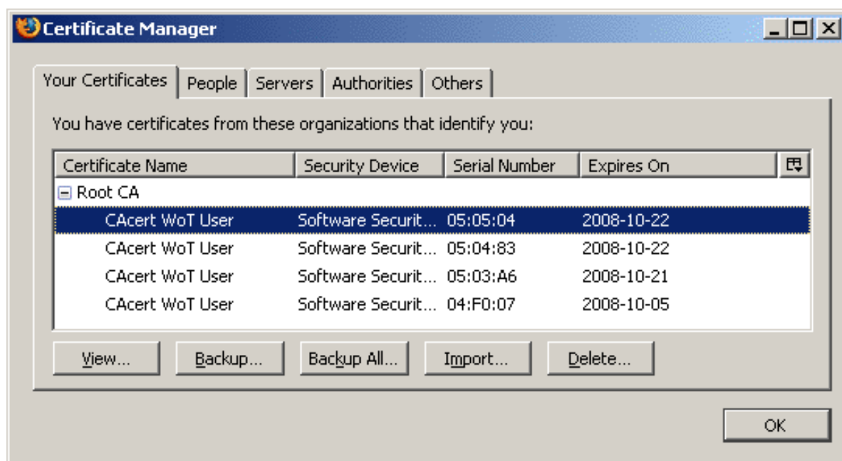
Figure 5.14. Certificate Manager
