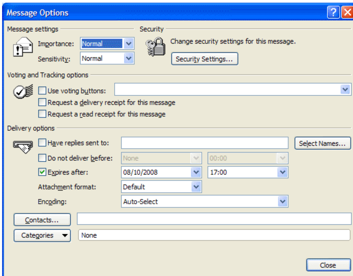
Figure 5.22. Message options
